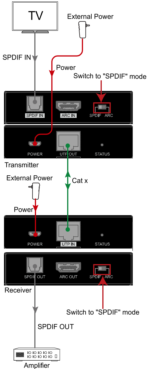
Figure 2 SPDIF Mode
