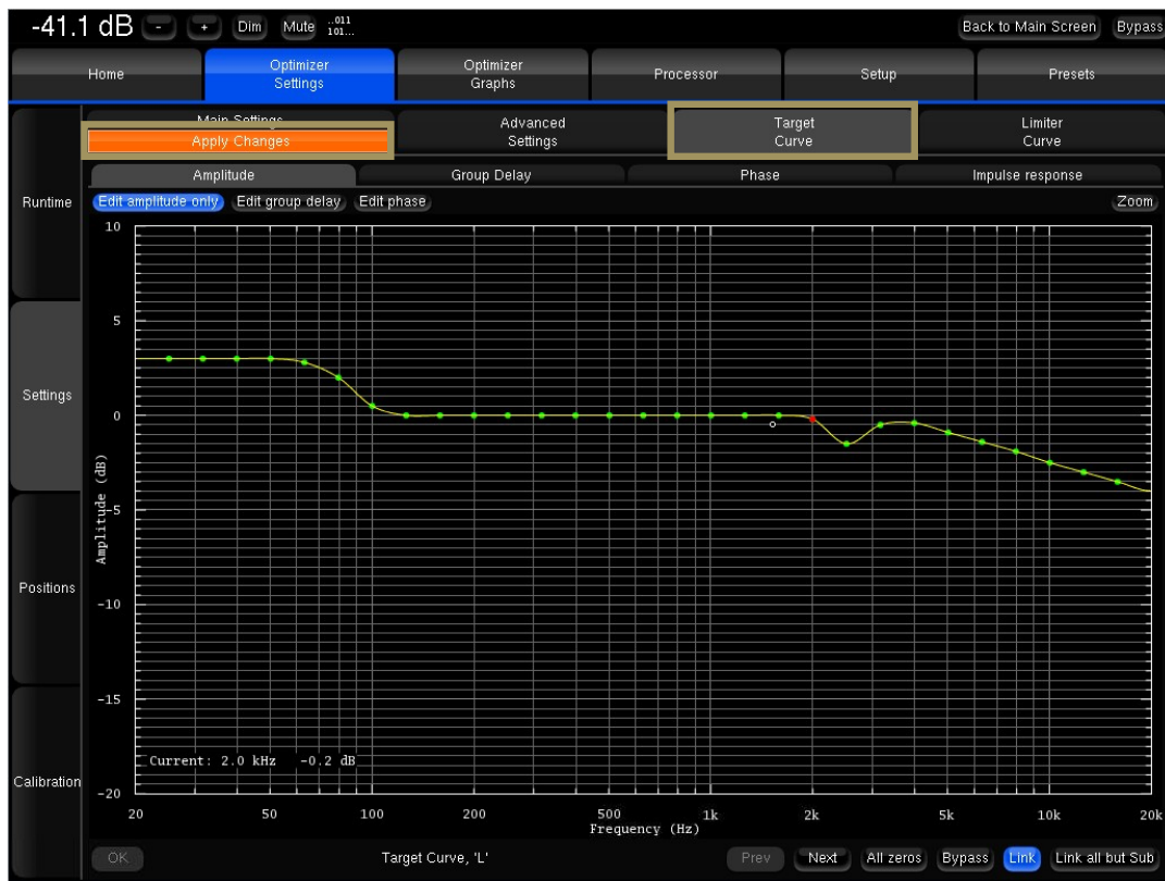
Figure 100: Example of a Target Curve in the Advanced Settings user interface
