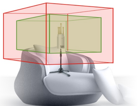
Figure 107: Relevant (green) / irrelevant (red) multi-point measurement area for a single listening position
