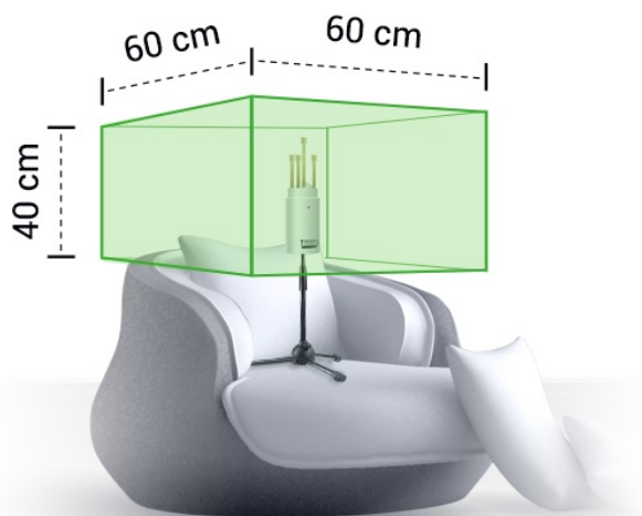
Figure 106: Relevant multi-point measurement area for a single listening position
